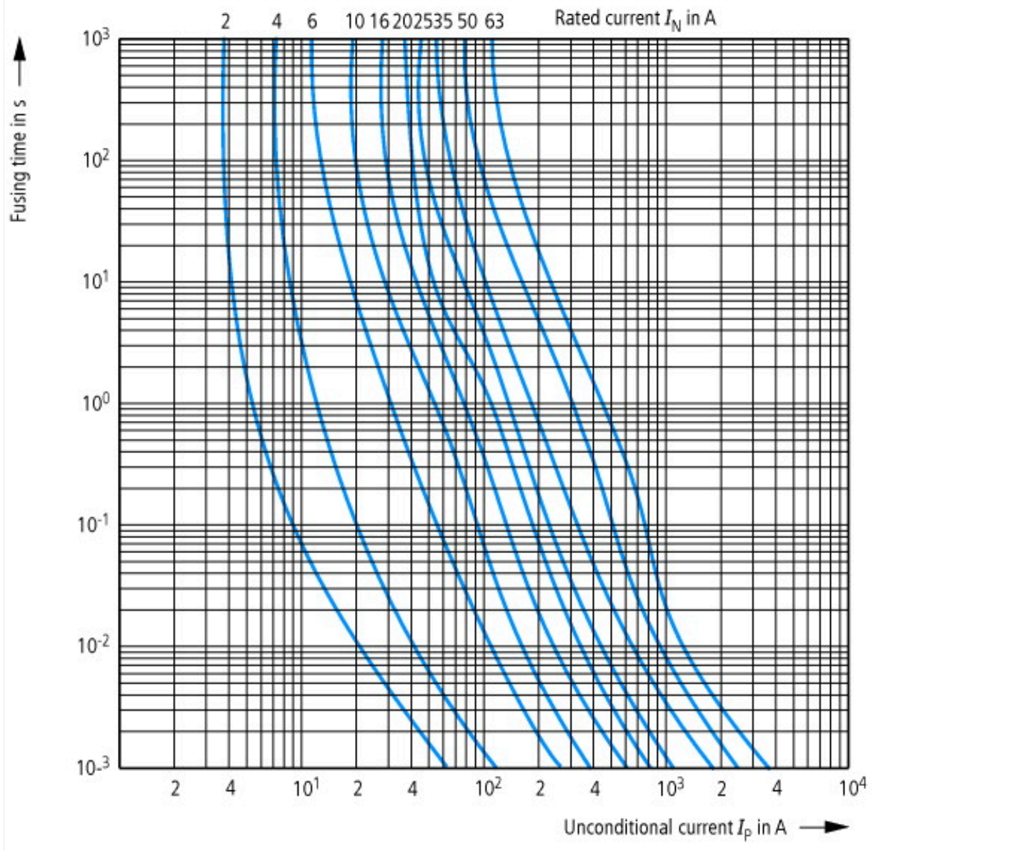
Let-through current characteristic curve
